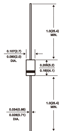
DO-41(DO-204AL)
